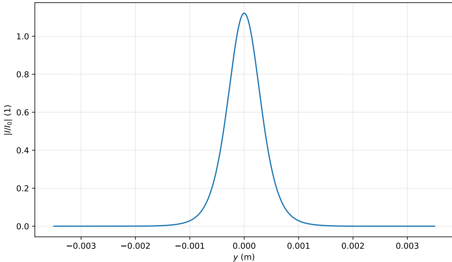
Intensity profile I(x=0, y, z=1.911)/I_0 , P_{in}=0.7P_{cr} , artificial time
